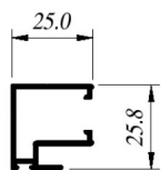
CIA-C147L Enganche ALN-147
