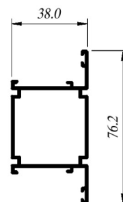
ALH-1103 Divisor
