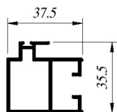
CIA-C191L Enganche ALN-191L
