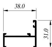
CIA-C173 Horizontal ALN-173
