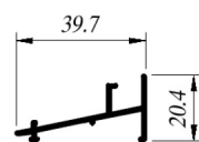
CIA-1630 Sillar
