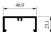
STO-B011 Horizontal
