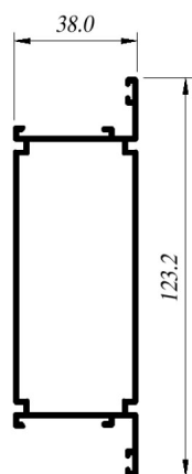
ALH-1104 Divisor
