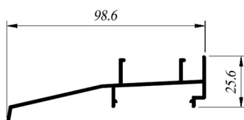
ALN-581 Sillar Alfajía ALN-581N
