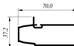
CIA-M2302 Divisor
