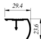
CIA-S-390 Remate
