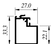
CIA-M156-M2 Enganche
