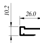
IND-001 Marco Polic
