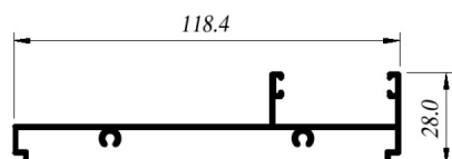
ALN-708M Jamba 3 Rieles ALN-708
