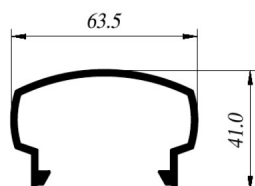
STO-B010 Pasamanos
