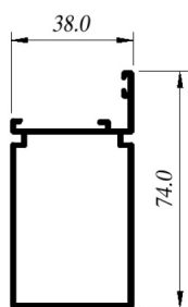
ALH-1734 Marco
