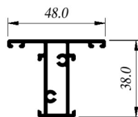
CIA-C292 Divisor ALN-292
