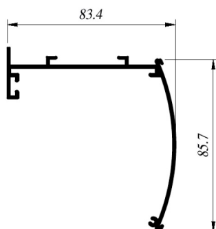
CIA-Co051L Cenefa
