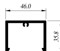
STO-B012 Vertical
