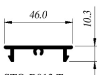
STO-B013 Tapa
