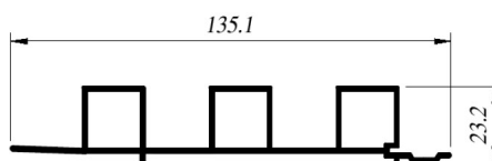
CIA-CH2554 Enchape
