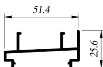
CIA-C194L Sillar ALN-194
